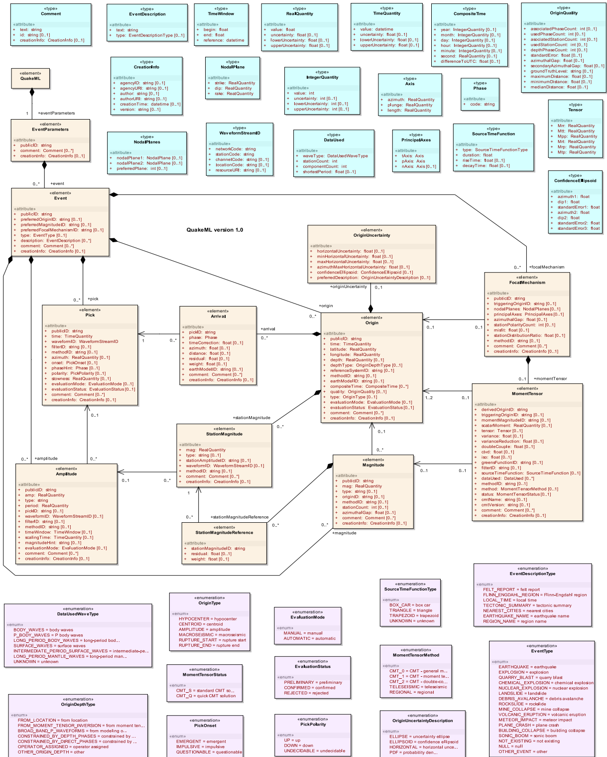
Figure 1: UML class diagram of the QuakeML data model. Two different types of relations between classes are used: (i) compositions, marked by lines with filled diamonds; and (ii) associations, marked by arrows. Compositions indicate a stronger coupling between two classes than associations.
