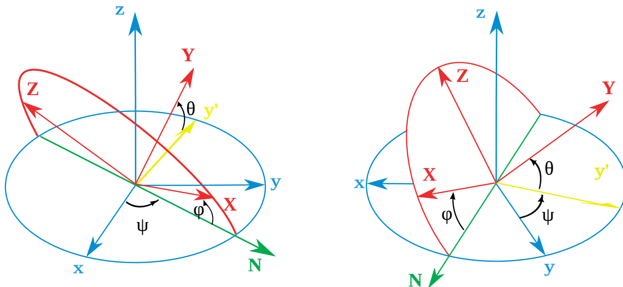
Figure 4: Definition of Tait-Bryan angles. Figure copyright by Juansempere, published under the Creative Commons Attribution 3.0 Unported license. Source: Wikipedia, http://en.wikipedia.org/wiki/Euler_angles
